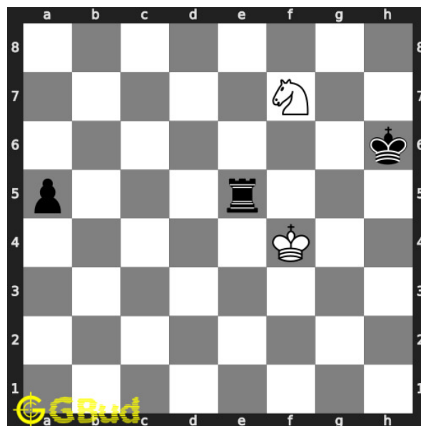
Figure 5: Nf7+
